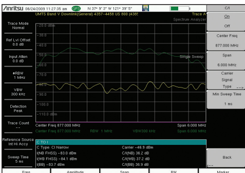
Carrier-to-Interference (C/I)
